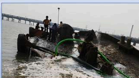
Pumping & De-watering
